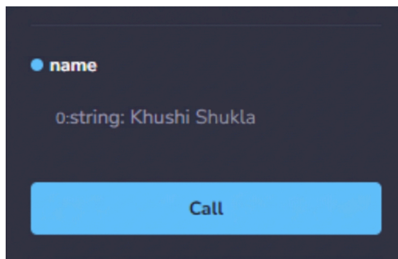
Figure 25: Practical screenshot
