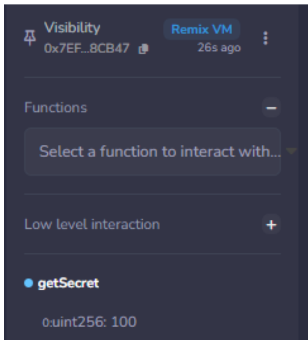
Figure 15: Practical screenshot
