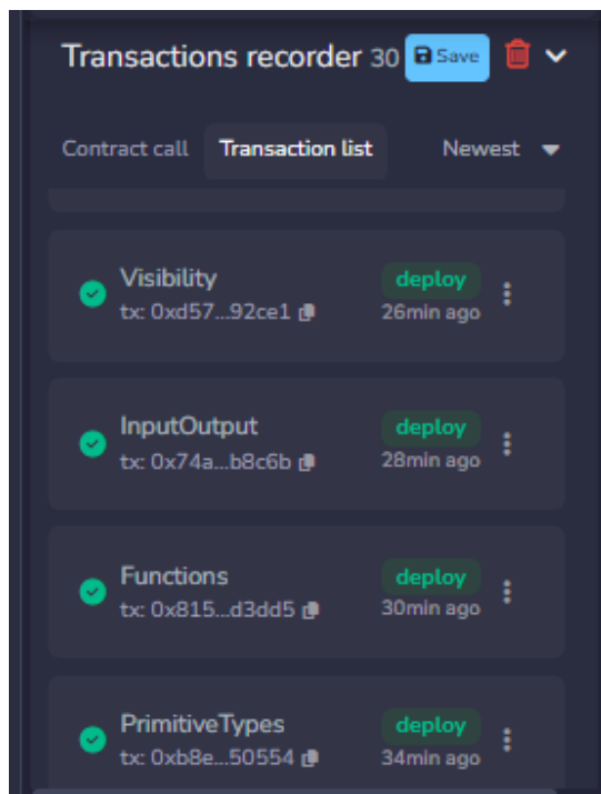
Figure 24: Practical screenshot
