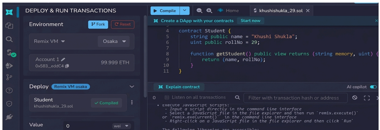
Figure 25: Practical screenshot
