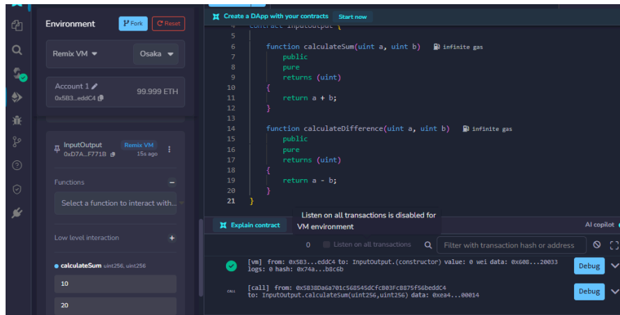
Figure 39: Practical screenshot
