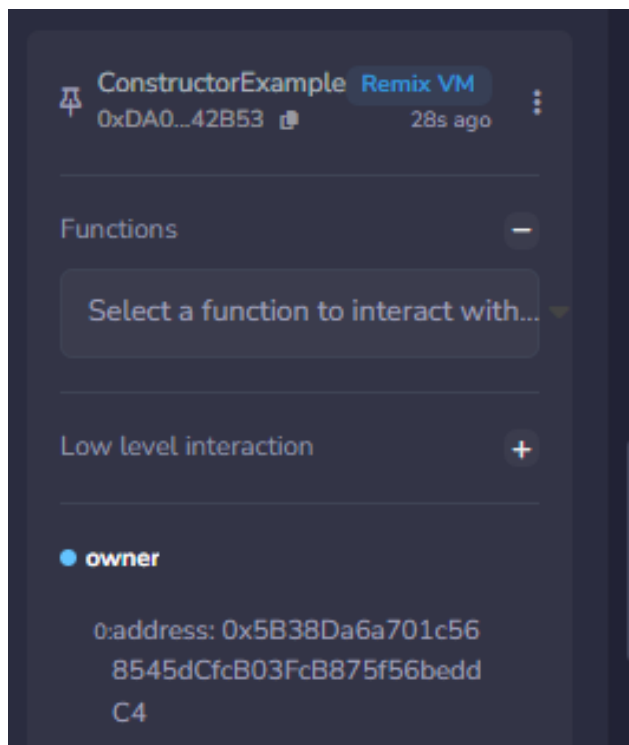
Figure 27: Practical screenshot
