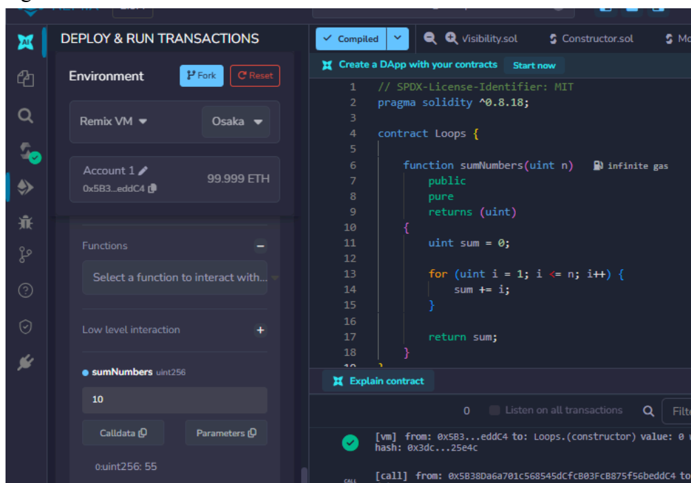
Figure 13: Practical screenshot
