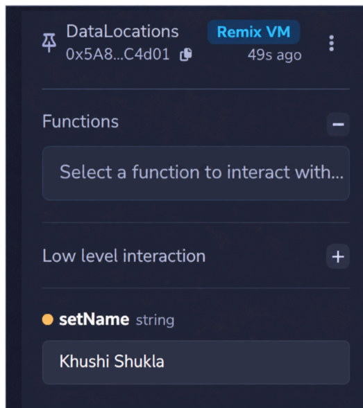
Figure 6: Practical screenshot
