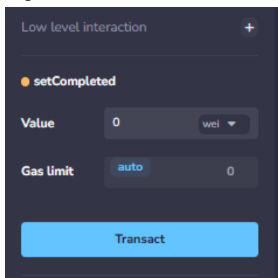
Figure 37: Practical screenshot
