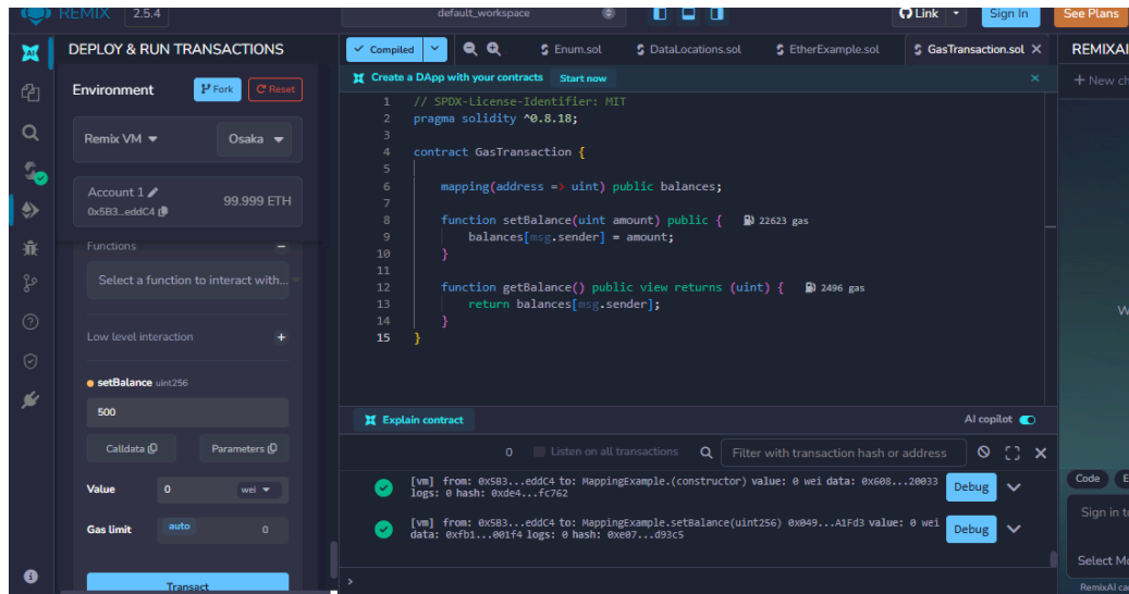
Figure 31: Practical screenshot
