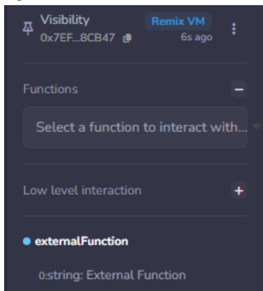
Figure 28: Practical screenshot
