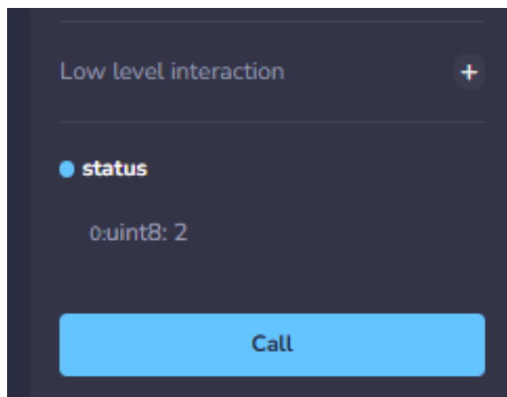
Figure 36: Practical screenshot
