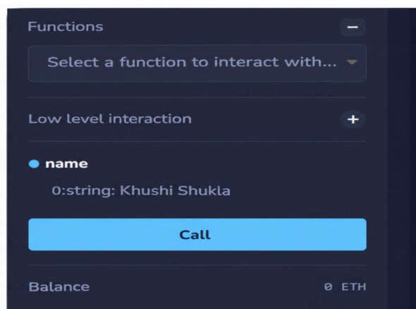
Figure 13: Practical screenshot
