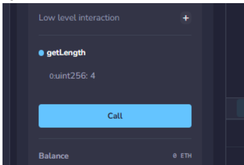
Figure 34: Practical screenshot
