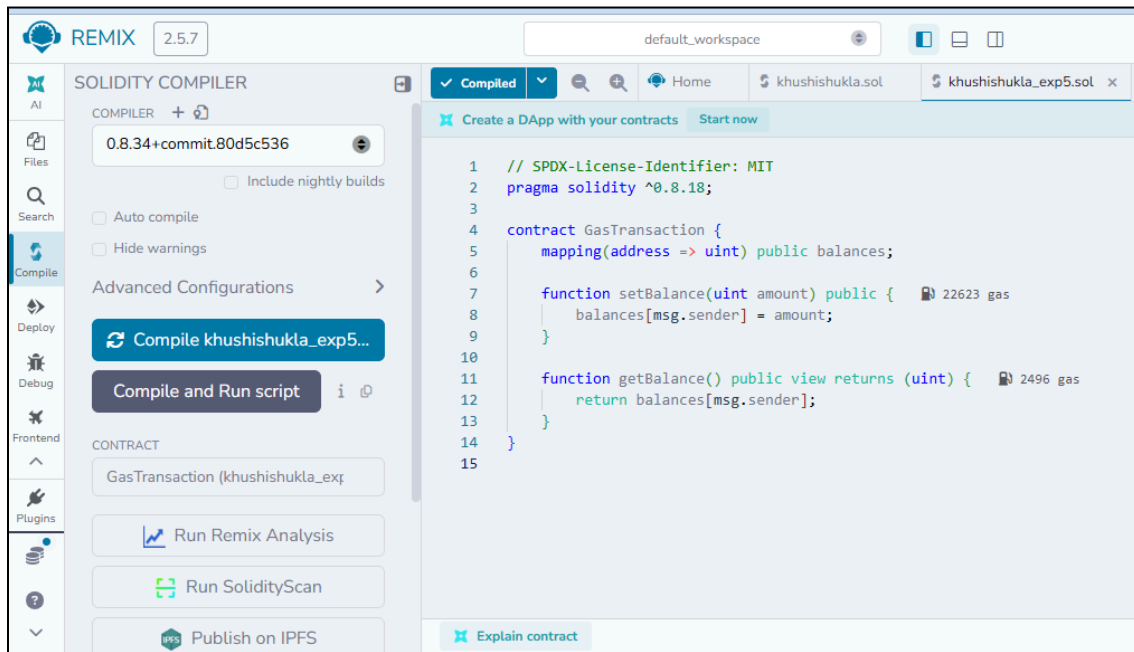
Figure 1: Practical screenshot
