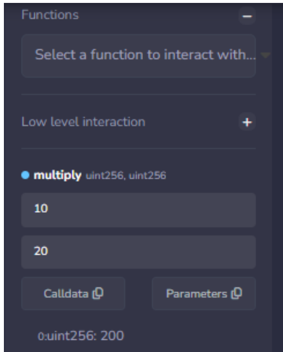
Figure 40: Practical screenshot
