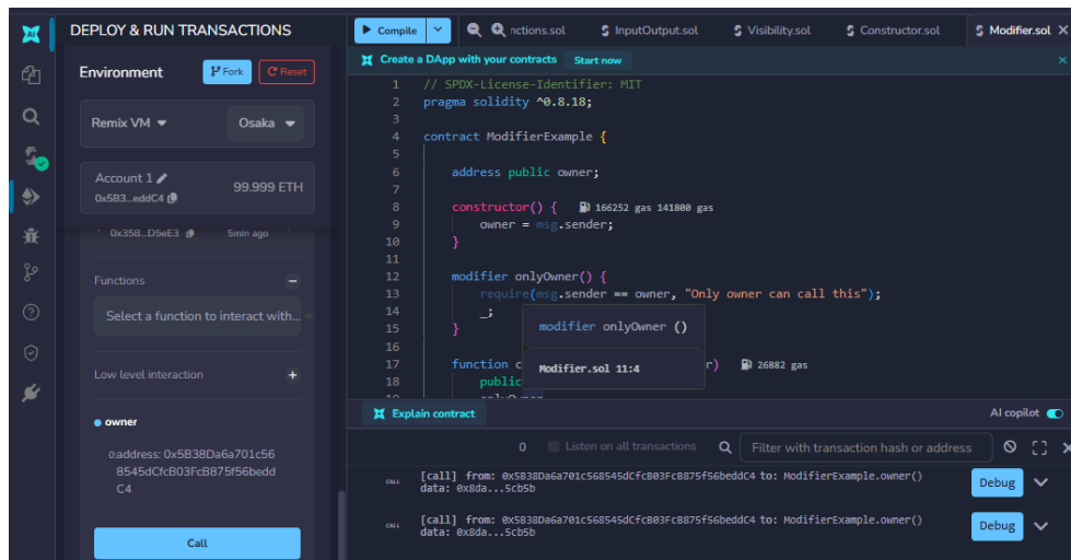
Figure 22: Practical screenshot
