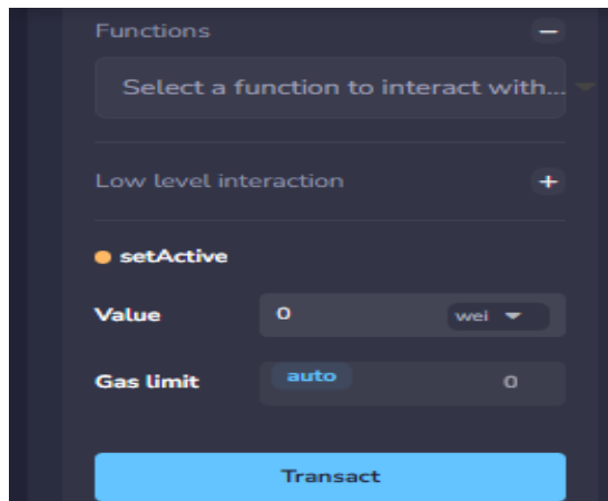
Figure 4: Practical screenshot
