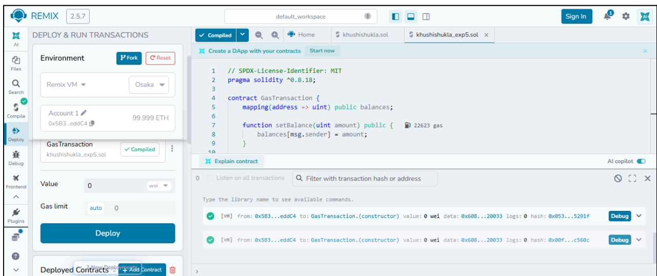
Figure 1: Practical screenshot
