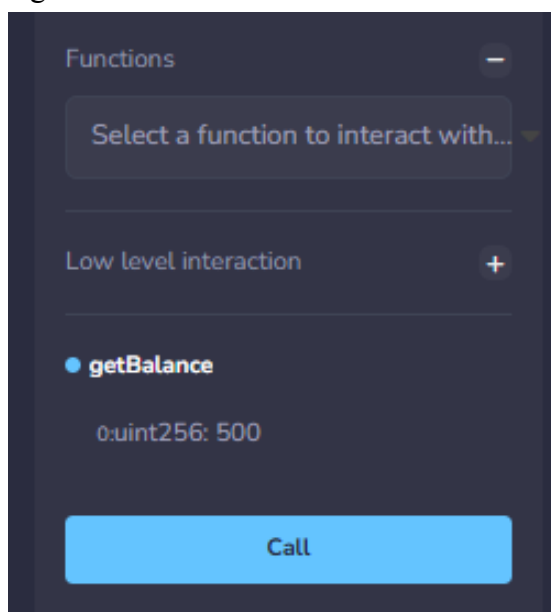
Figure 19: Practical screenshot
