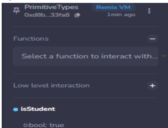
Figure 7: Practical screenshot
