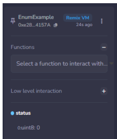
Figure 16: Practical screenshot
