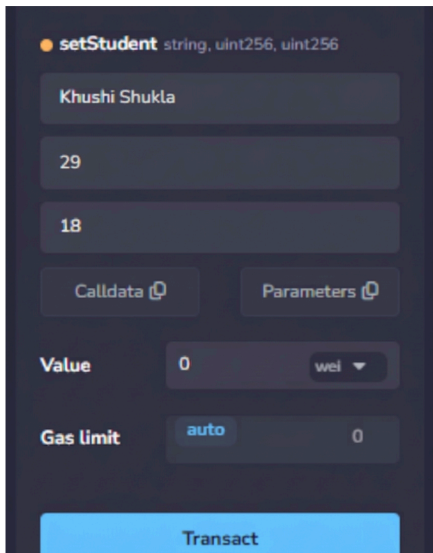
Figure 31: Practical screenshot
