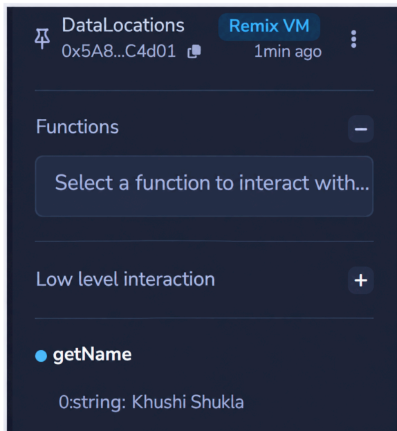
Figure 3: Practical screenshot
