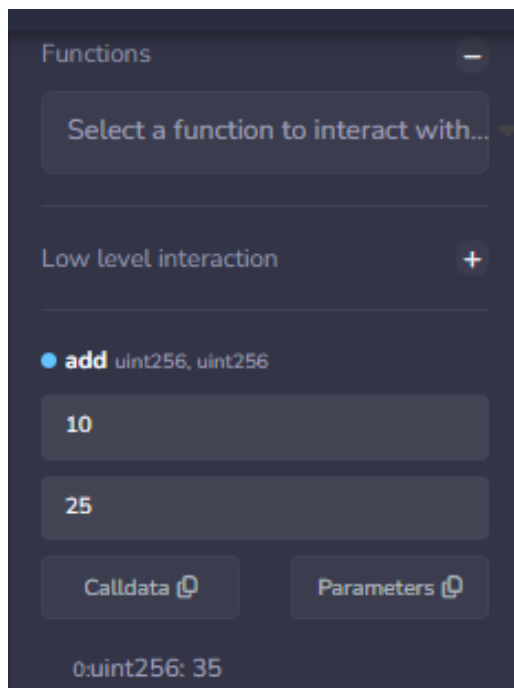
Figure 37: Practical screenshot
