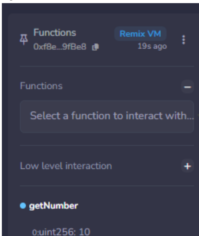
Figure 10: Practical screenshot
