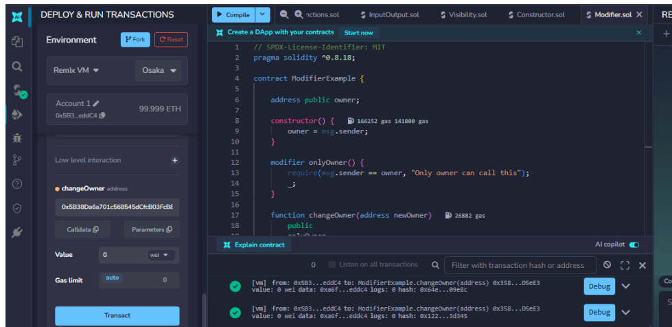
Figure 22: Practical screenshot
