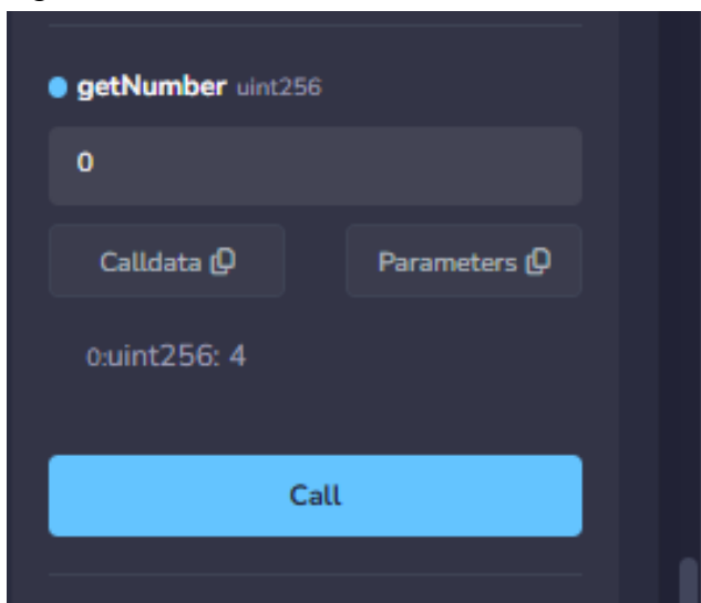
Figure 7: Practical screenshot
