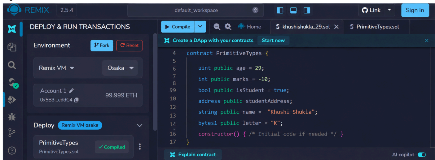
Figure 9: Practical screenshot
