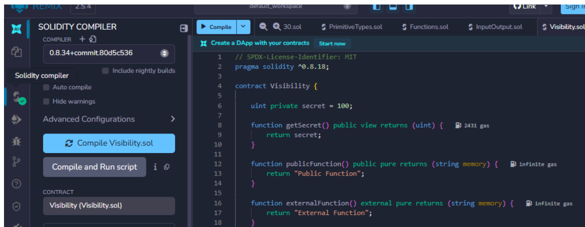
Figure 4: Practical screenshot
