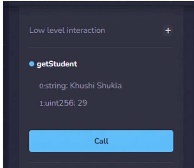
Figure 21: Practical screenshot
