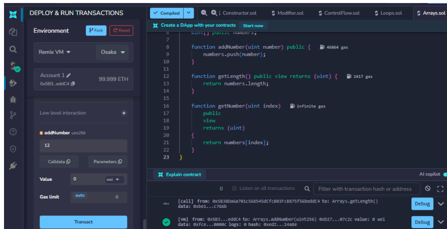
Figure 33: Practical screenshot
