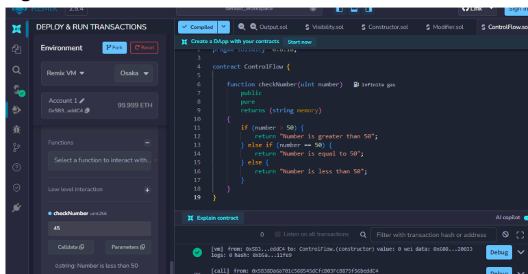
Figure 18: Practical screenshot
