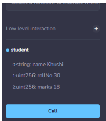
Figure 10: Practical screenshot
