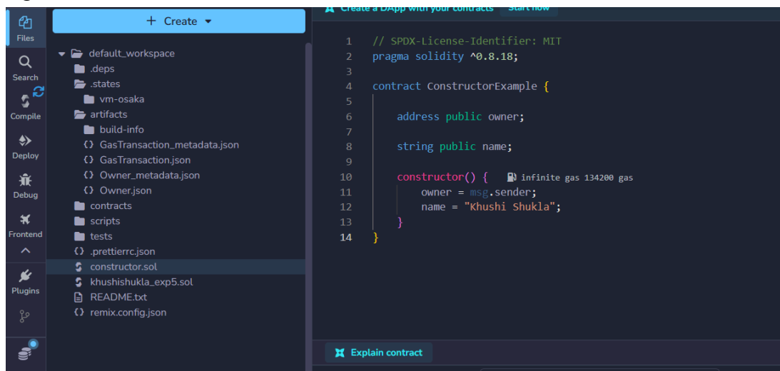
Figure 16: Practical screenshot
