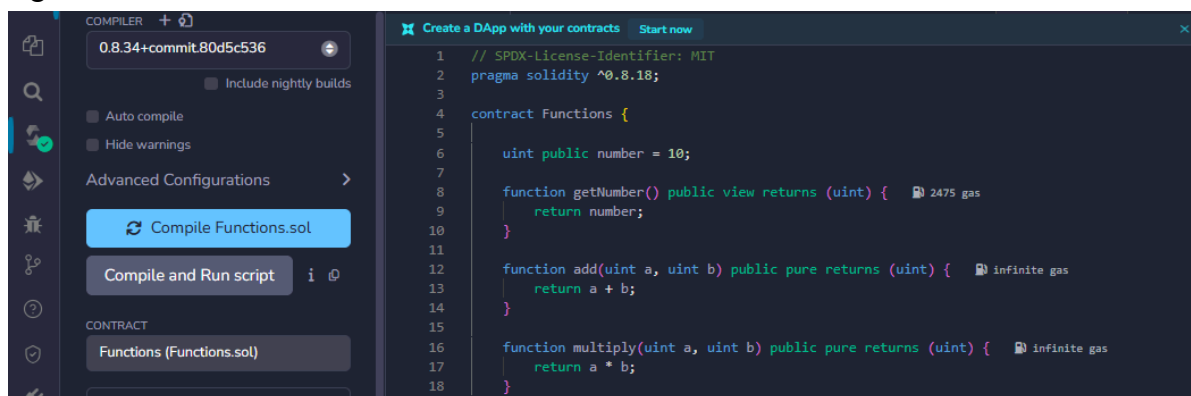
Figure 12: Practical screenshot
