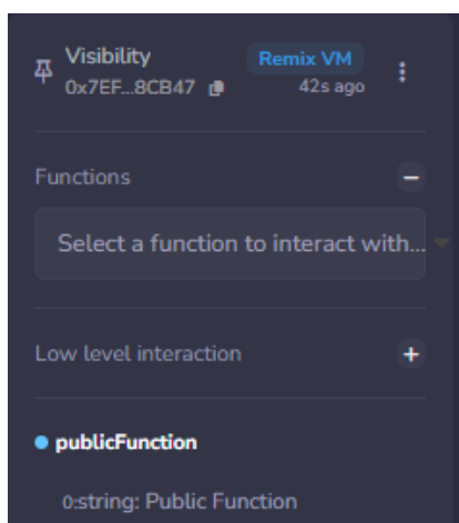
Figure 20: Practical screenshot
