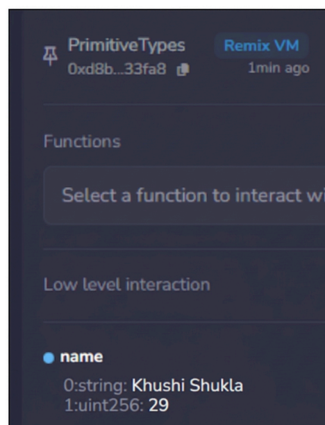
Figure 34: Practical screenshot
