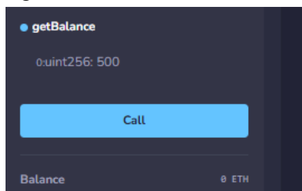
Figure 28: Practical screenshot
