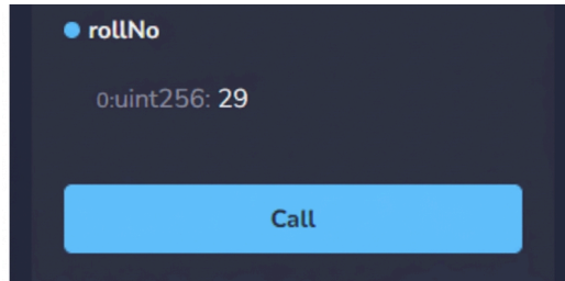
Figure 30: Practical screenshot
